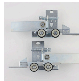
电梯层门锁 M2Z(T)S8
