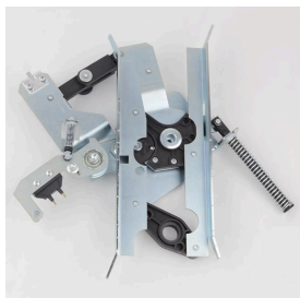
电梯门刀 KM900650G13
