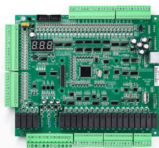
电梯Main Board MCTC-MCB-H
