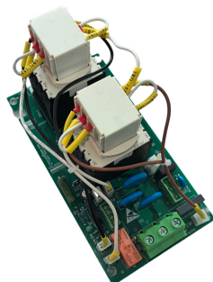
电梯Contactor Board KM964619G24
