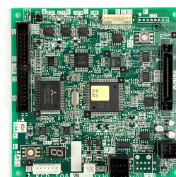
电梯Main Board KCD-1060B
