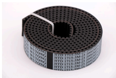
电梯Door Machine Belt HTD 1715-5M-25
