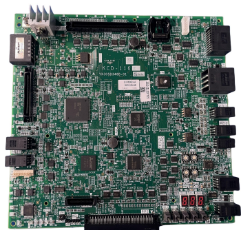
电梯Main Board KCD-1161D
