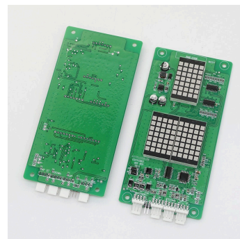
电梯Display Board MCTC-HCB-R4
